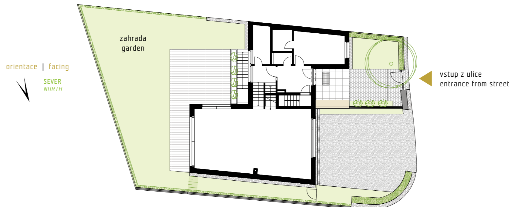
1NP a pozemek | 1 st floor and plot
